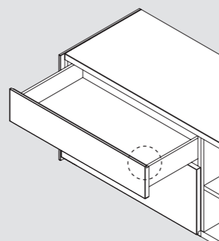
Detalle galce frentes AddLiving
