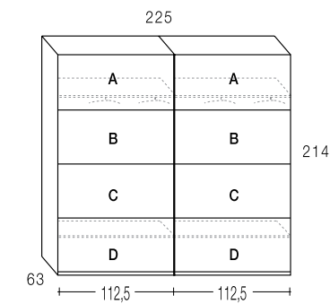
Ref. DK46 Armario corredero 2 puertas
